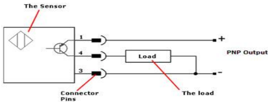
PNP 3-wire Standard Diagram
